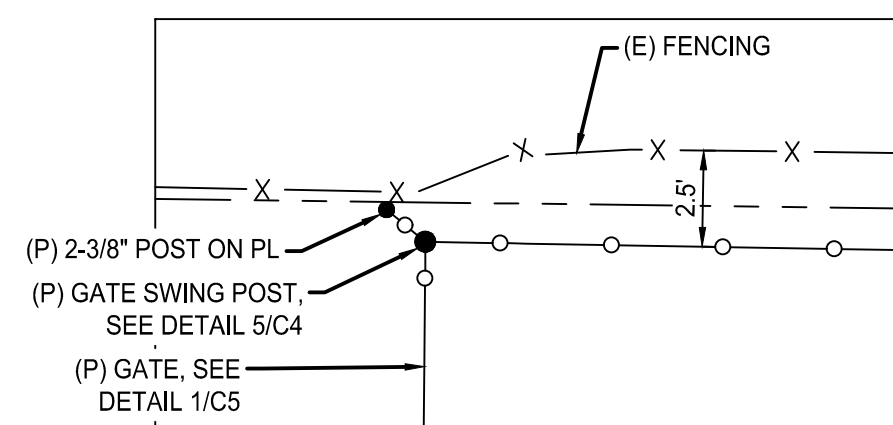
B C3 FENCE DETAIL NTS
