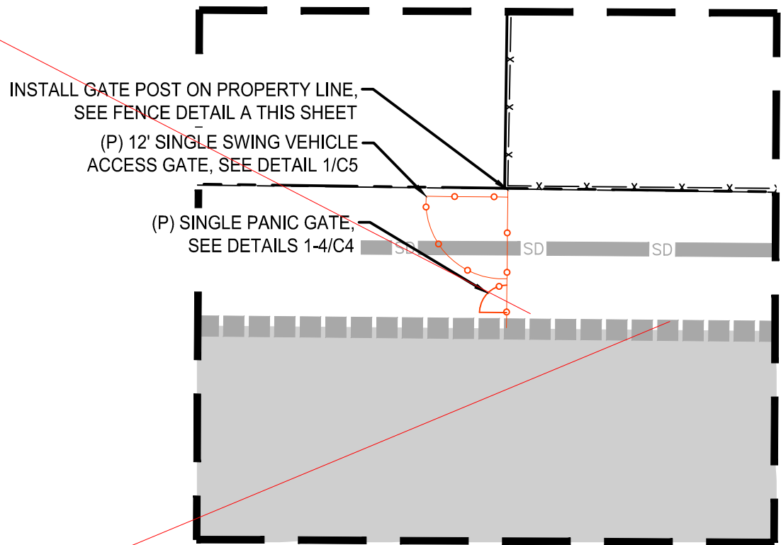
DETAILED SITE PLAN 1 SCALE: 1" = 20'
