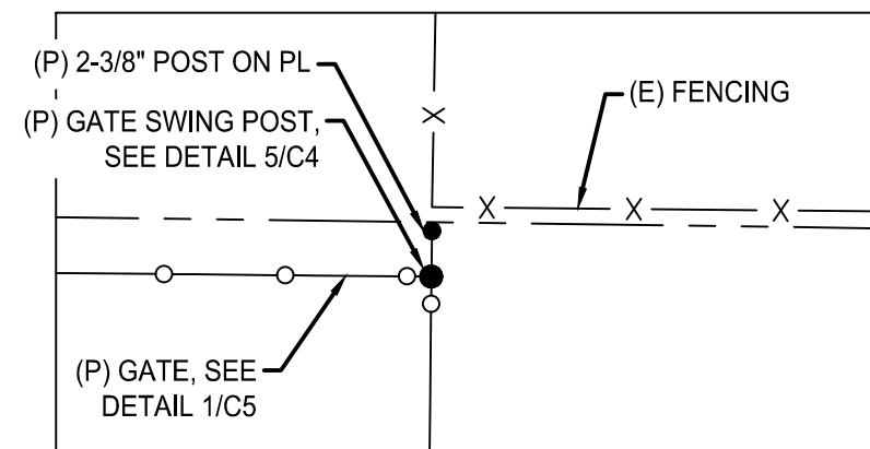
A C3 FENCE DETAIL NTS
