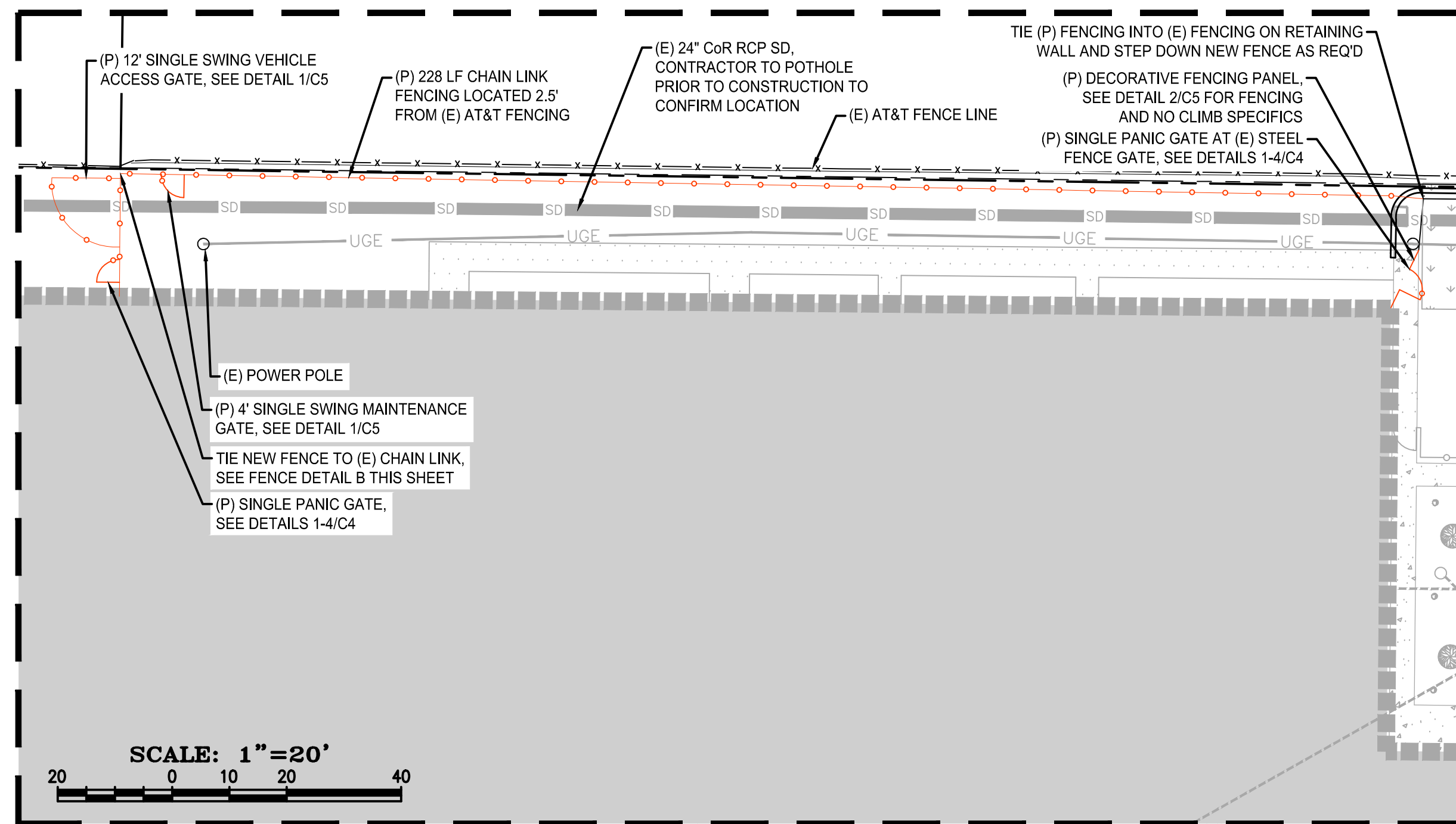
DETAILED SITE PLAN 2 SCALE: 1" = 20'
