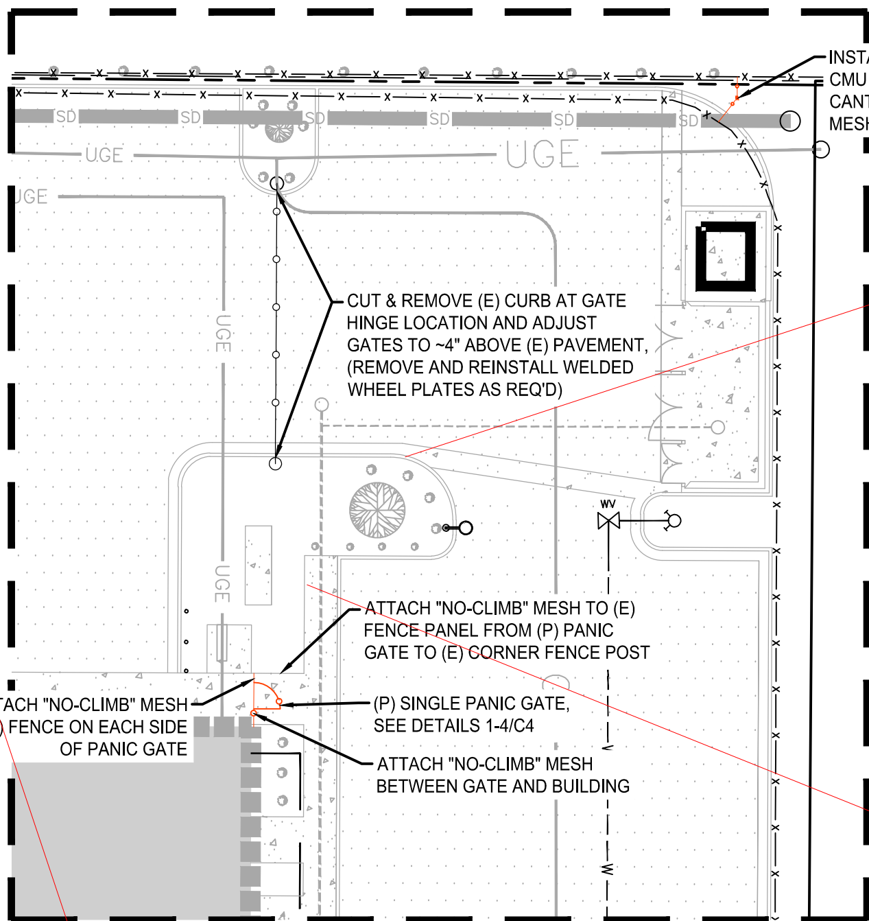
DETAILED SITE PLAN 3 SCALE: 1" = 20'
