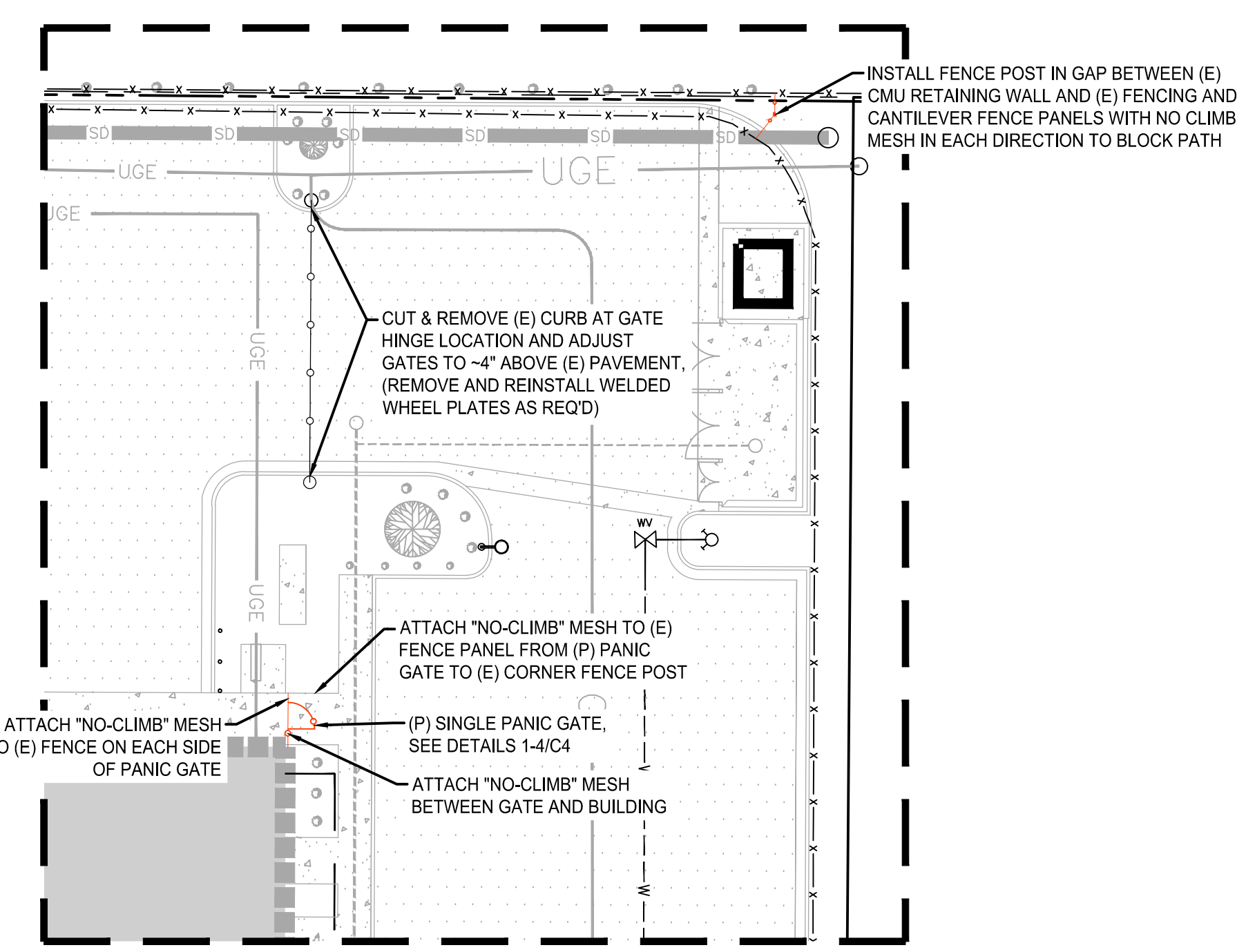
DETAILED SITE PLAN 3 SCALE: 1" = 20'
