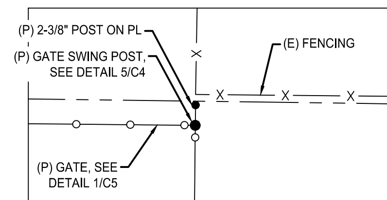
A C3 FENCE DETAIL NTS
