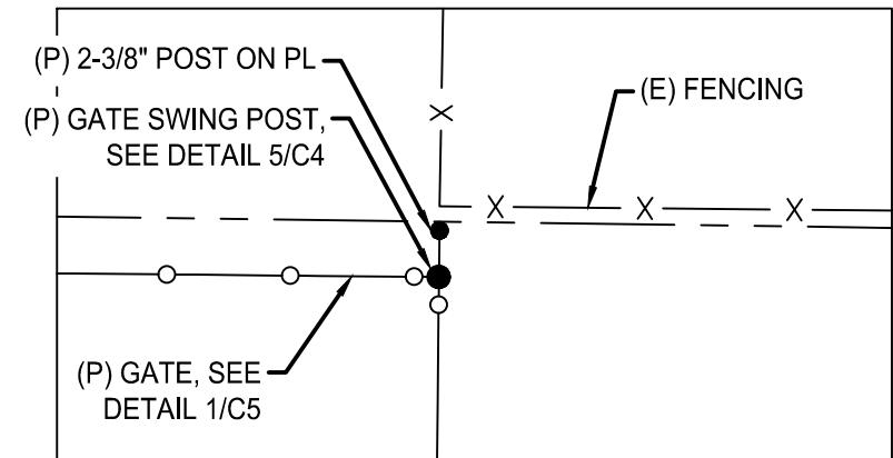
A C3 FENCE DETAIL NTS
