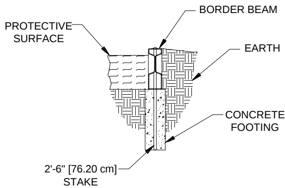
3790/3791 BELOW GRADE
