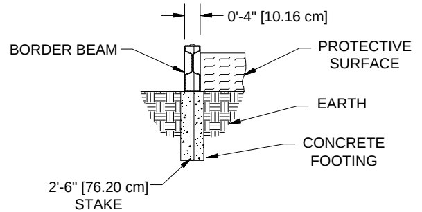
3790/3791 ABOVE GRADE
