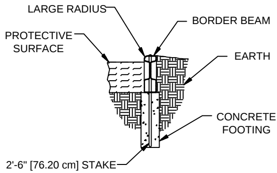
3781/3783/3792/3793 BELOW GRADE
