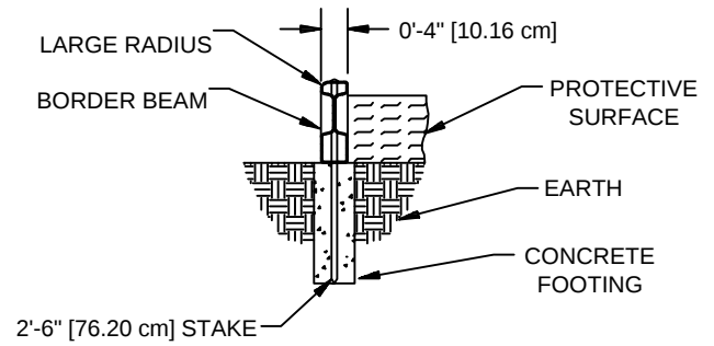
3781/3783/3792/3793 ABOVE GRADE
